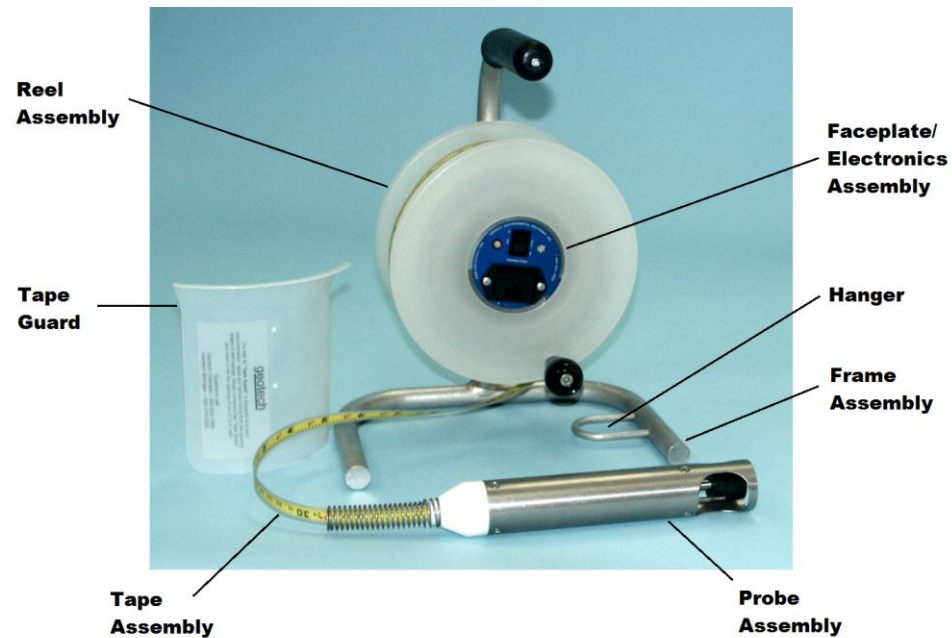
Figure 1-1 – System Components
